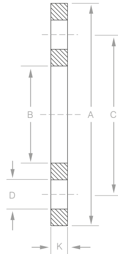
SS Backing Ring
