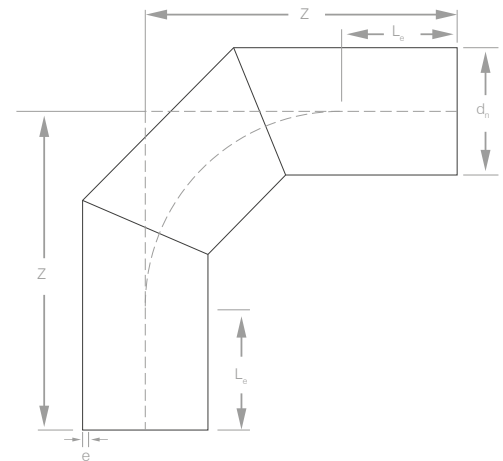
90° Elbow
