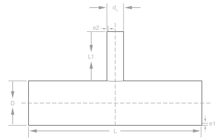
Reducer Tee
